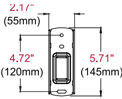
WALL PLATE DETAIL
