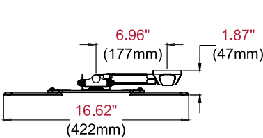
TOP VIEW COLLAPSED
