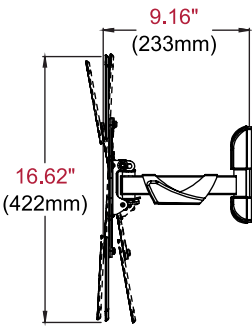
SIDE VIEW +10°/-3° TILT
