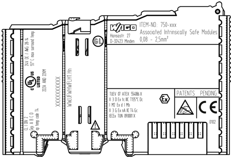
Figure 49: Marking Example According to NEC
