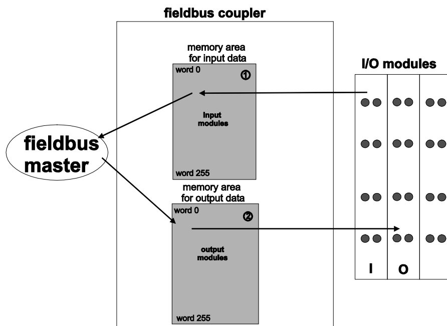
Figure 37: Memory Areas and Data Exchange
