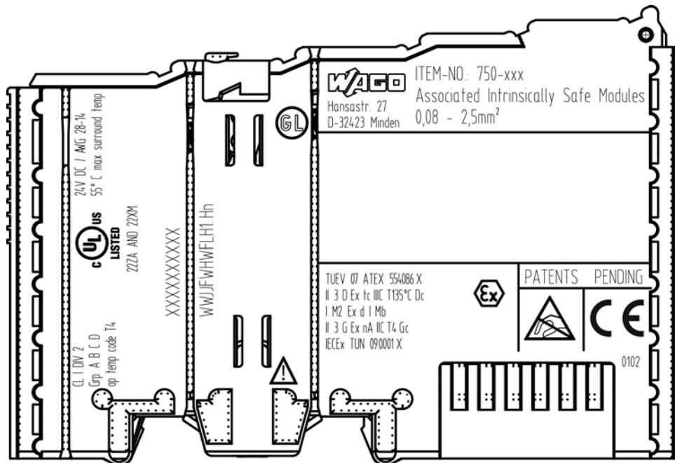
Figure 45: Marking Example According to ATEX and IECEx
