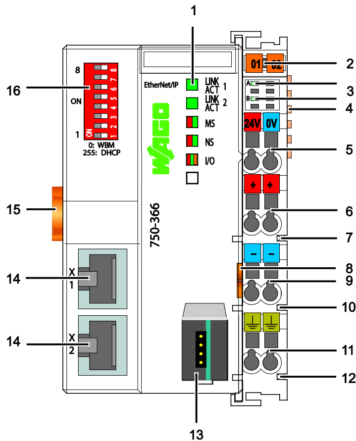
Figure 22: View Controller EtherNet/IP; G4; DLR
