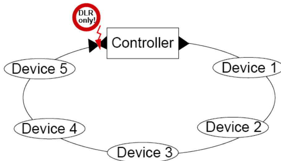
Figure 43: DLR ring with closed port, one line for EtherNet/IP communication
