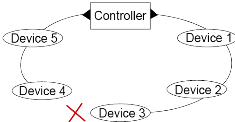
Figure 44: DLR ring with an interruption (between device 3 and 4), two lines for EtherNet/IP communication
