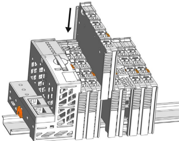
Figure 31: Snap the I/O Module into Place (Example)
