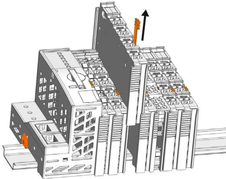
Figure 32: Removing the I/O Module (Example)
