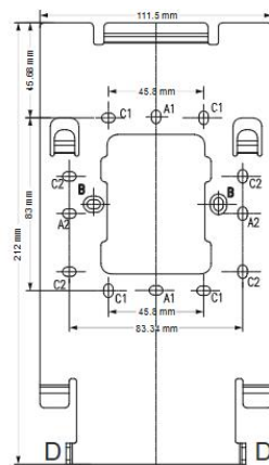
Bracket hole position diagram
