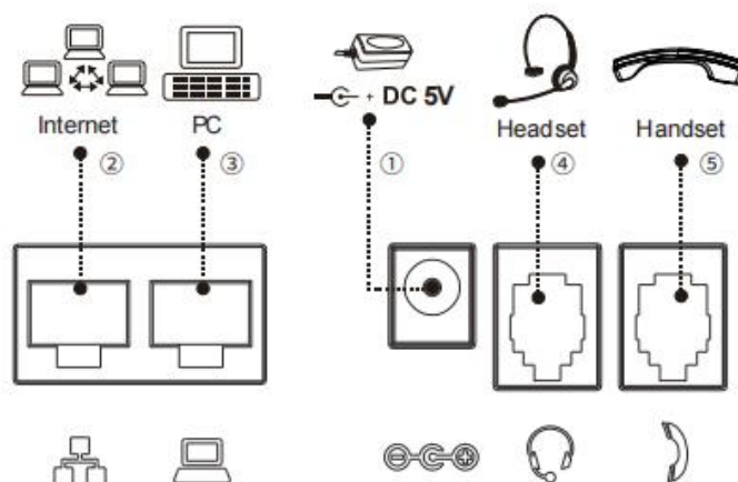
Picture 3 - Connecting to the Device
