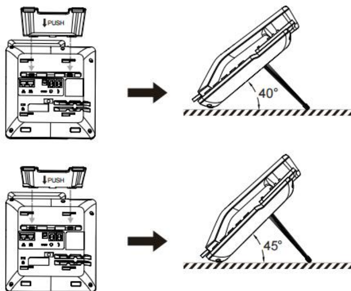
Picture 1 - Device installation
