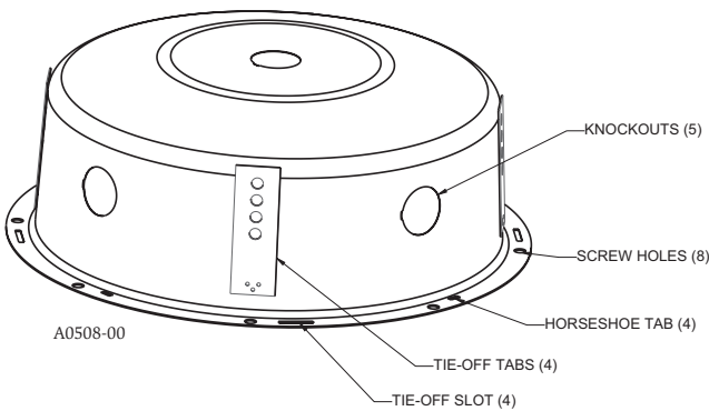
FIGURE 3 BACK CAN
