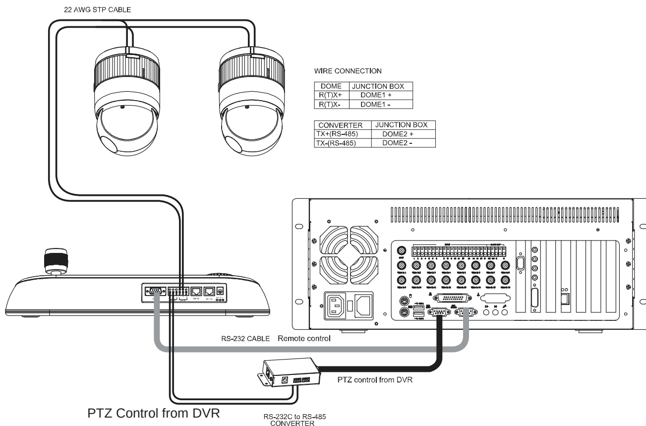
Figure 11 – PC DVR Connection Diagram
